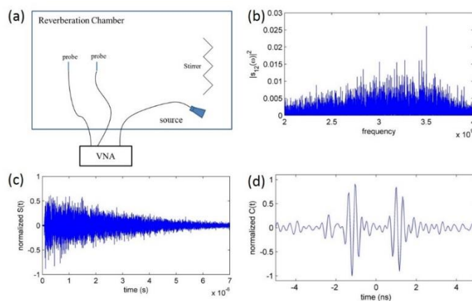
Fig : (a) Setup used for Green's function retrieval. Two non-invasive probes record the field transmitted by a source antenna located in the RC. (b) Spectrum between 2 and 4 GHz of the transmission coefficient between the source antenna and the first receiving antenna. (c) Impulse response which is the inverse Fourier transform of s_{13}(\omega) . (d) Cross-correlation C(t) of the field probed at two positions. The cross-correlation converges towards the coherent response between the antennas.
